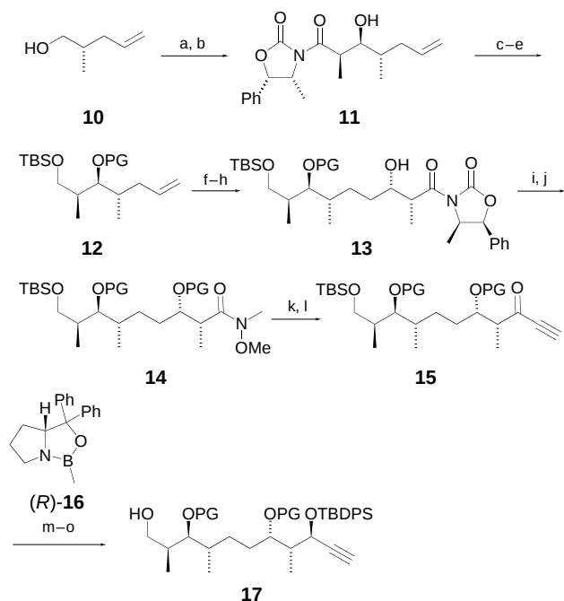
Scheme 2. Synthesis of intermediate 17 , which incorporates all stereogenic centers. a) (COCl) 2 , DMSO, NEt 3 , CH 2 Cl 2 , –78 °C → RT; b) 7 , Bu 2 BOTf, DIPEA, CH 2 Cl 2 , –78 °C → RT, then H 2 O 2 , pH 7, 0 °C → RT, 68 % over two steps; c) MOMCl, DIPEA, CH 2 Cl 2 , room temperature, 97 %; d) LiBH 4 , H 2 O, Et 2 O, 0 °C → RT, 78 %; e) TBSCl, imidazole, DMF, room temperature, 97 %; f) 9-BBN, THF, room temperature, then H 2 O 2 , NaOH, 83 %; g) (COCl) 2 , DMSO, NEt 3 , CH 2 Cl 2 , –78 °C → RT; h) 7 , Bu 2 BOTf, DIPEA, CH 2 Cl 2 , –78 °C → RT, then H 2 O 2 , pH 7, 0 °C → RT; TBSCl, NEt 3 , DMAP, CH 2 Cl 2 , room temperature, 86 % over two steps; i) Me 3 Al, (H 2 NMeOMe) + Cl – , THF, –10 °C → 0 °C, 84 %; j) MOMCl, DIPEA, CH 2 Cl 2 , room temperature, 92 %; k) 9 , BuLi, –78 °C; THF, –78 °C → –10 °C; l) borax, methanol, H 2 O, –10 °C → RT, 95 % over two steps; m) ( R )- 16 , BH 3 ·Me 2 S, THF, –30 °C, 96 %; n) TBDPSCl, imidazole, DMF, room temperature; o) HF/pyridine, THF, room temperature, 40 min, 88 % over two steps. DMSO = dimethyl sulfoxide, Tf = trifluoromethanesulfonyl, DIPEA = diisopropylethylamine, DMF = N,N -dimethylformamide, 9-BBN = borabicyclo[3.3.1]nonane, DMAP = 4-dimethylaminopyridine, PG = protecting group = MOM = methoxymethyl.
