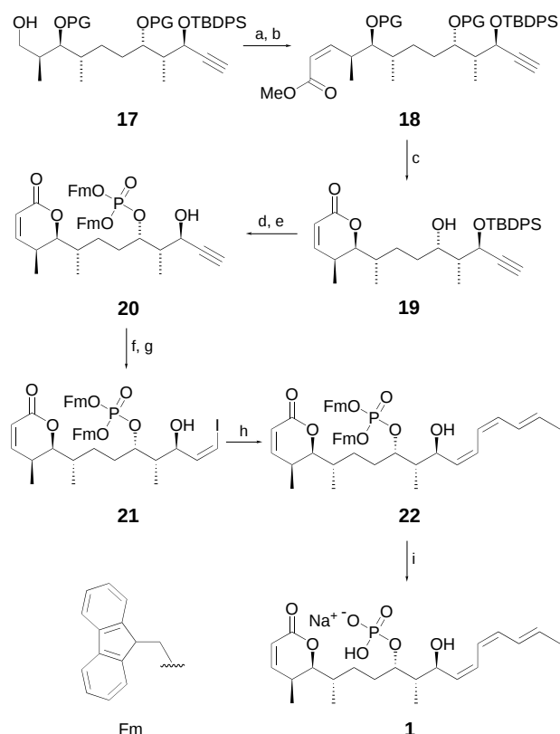
Scheme 3. Synthesis of 1 . a) DMP, \text{CH}_2\text{Cl}_2 , \text{NaHCO}_3 , 93%; b) (\text{CF}_3\text{CH}_2\text{O})_2\text{P}(\text{O})\text{CH}_2\text{CO}_2\text{Me} , [18]crown-6, KHMDs, THF, -78^\circ\text{C} , 92%; c) \text{CBr}_4 , 2-propanol, 82^\circ\text{C} , 83%; d) (\text{FmO})_2\text{PNiPr}_2 , tetrazole, \text{CH}_2\text{Cl}_2/\text{CH}_3\text{CN} , 0^\circ\text{C} \rightarrow \text{RT} , then \text{I}_2 , pyridine, \text{H}_2\text{O} , THF; 95%; e) HF/pyridine, THF, room temperature, 28 h, 82%; f) NIS, \text{AgNO}_3 , DMF, room temperature, quant.; g) \text{K}^+\text{OOC-N=N-COO}^-\text{K}^+ , HOAc, 2-propanol/dioxane, 63%; h) 5 , [\text{PdCl}_2(\text{CH}_3\text{CN})_2] (cat.), DMF/THF, 62%; i) \text{NEt}_3:\text{CH}_3\text{CN} 1:5, room temperature, then \text{Na}^+\text{-Dowex resin} , 85%. DMP = Dess–Martin periodinane, HMDs = hexamethyldisilazane, NIS N -iodosuccinimide; PG = MOM.
