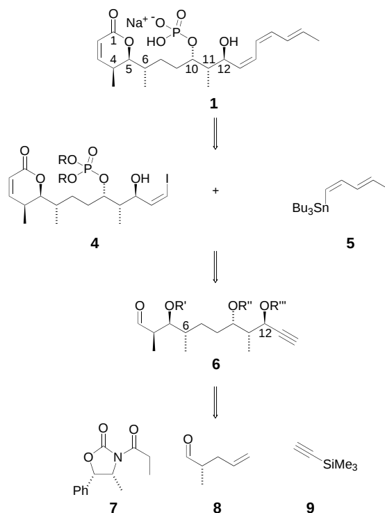
Scheme 1. Retrosynthetic analysis of (4 S ,5 S ,6 S ,10 S ,11 S ,12 S )-cytoestatin.
